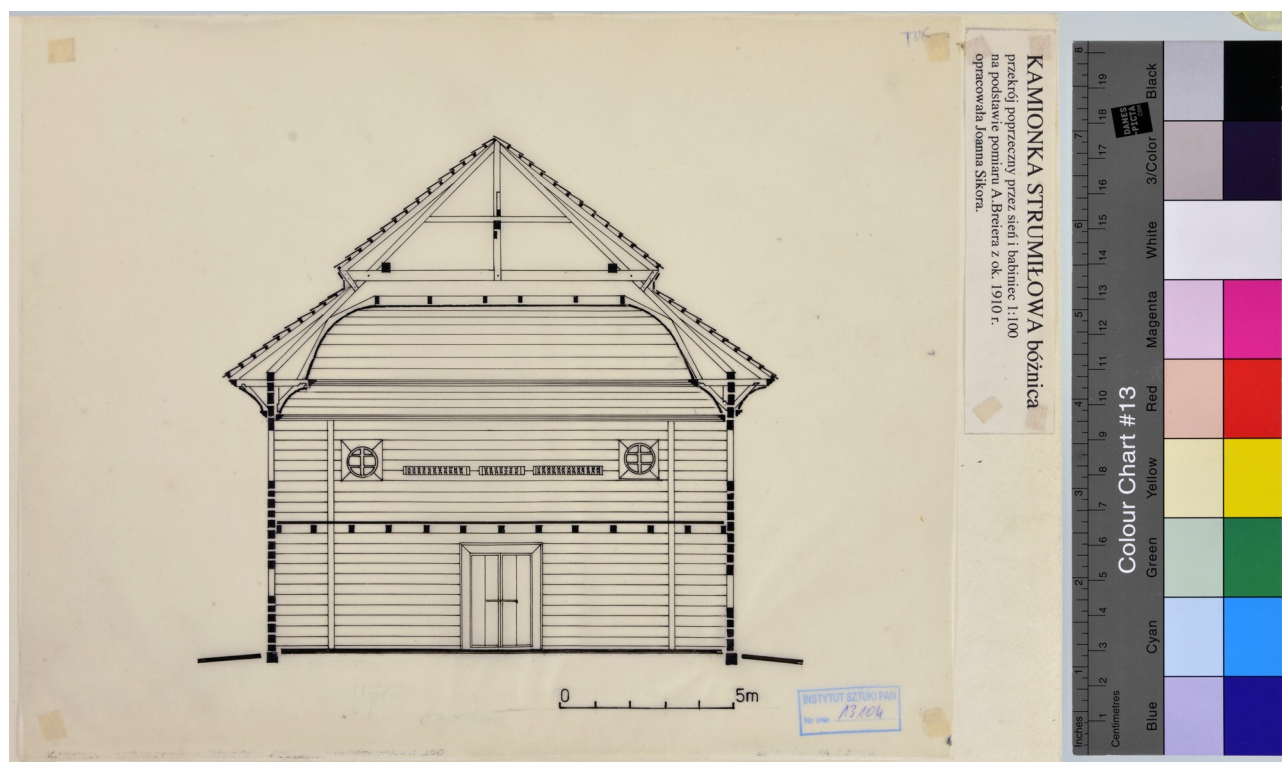
Fig. 3 Cross-section through the entrance hall and the women's room
