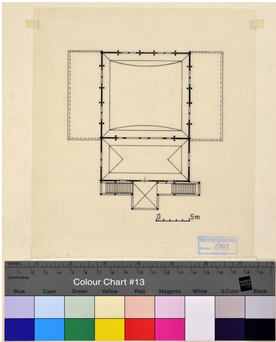
Fig. 8 Plan of the ceiling
