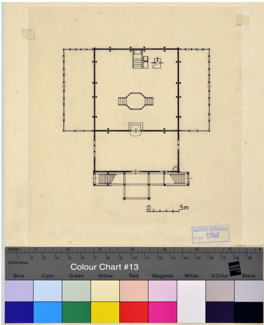
Fig. 7 Plan of 0 Floor
