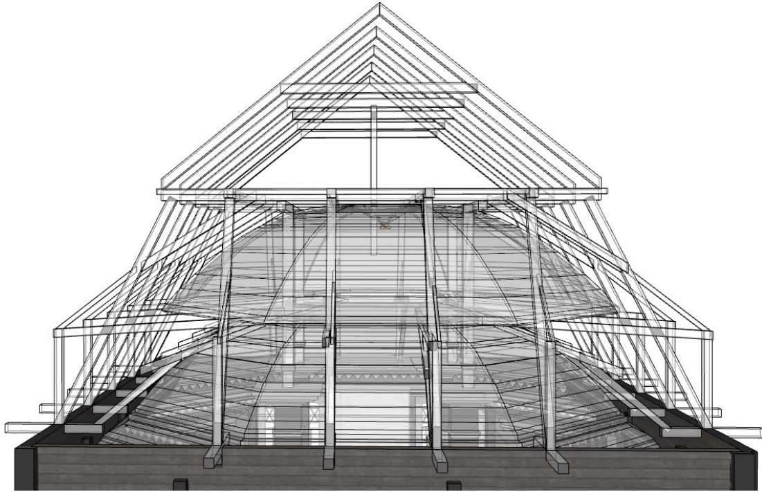
Fig. 16 Truss Roofing
