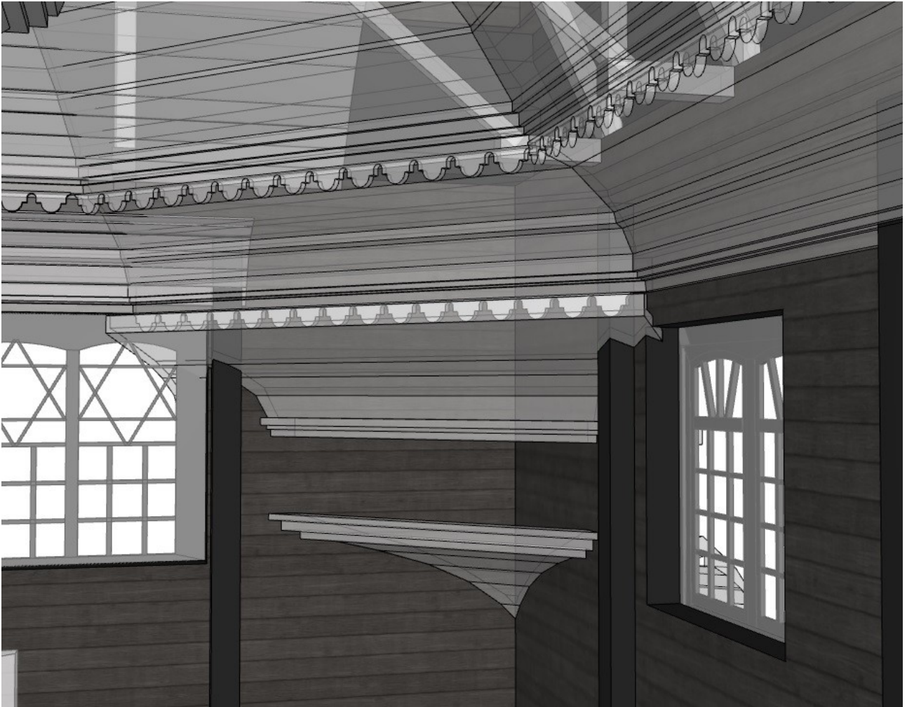
Fig. 41 Squinches_3D view
