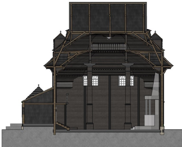
Fig. 56 2_section_with south wall in view.jpg
