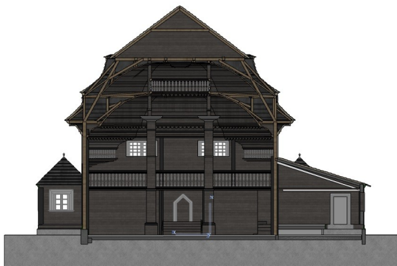
Fig. 57 2_section_with west wall in view.jpg
