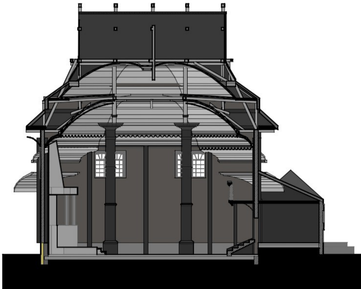
Fig. 27 section_with south wall in view.jpg
