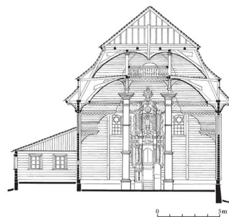
Fig. 6 533. Olkieniki. Section looking towards the east wall
