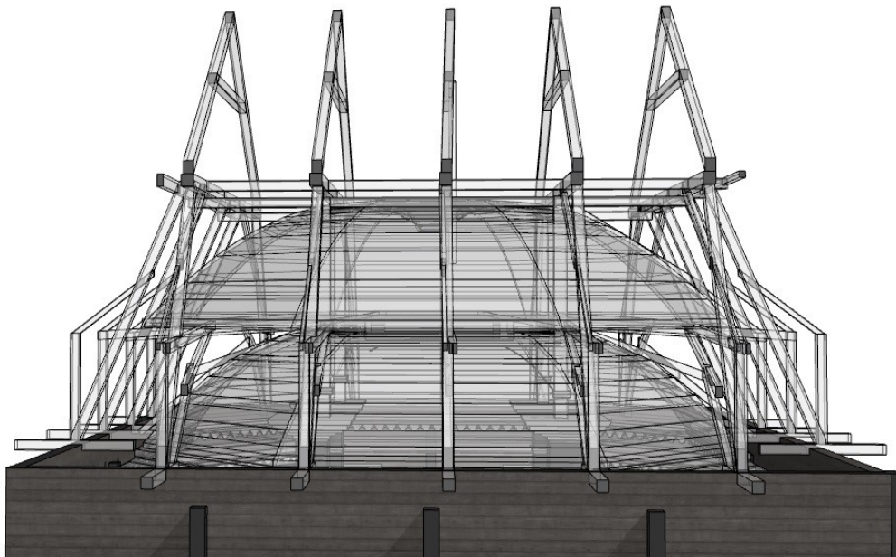
Fig. 18 Truss roofing_side view
