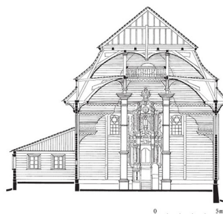
Fig. 6 533. Olkieniki. Section looking towards the east wall
