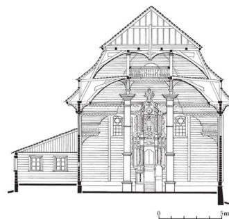
Fig. 6 533. Olkieni. Section looking towards the east wall
