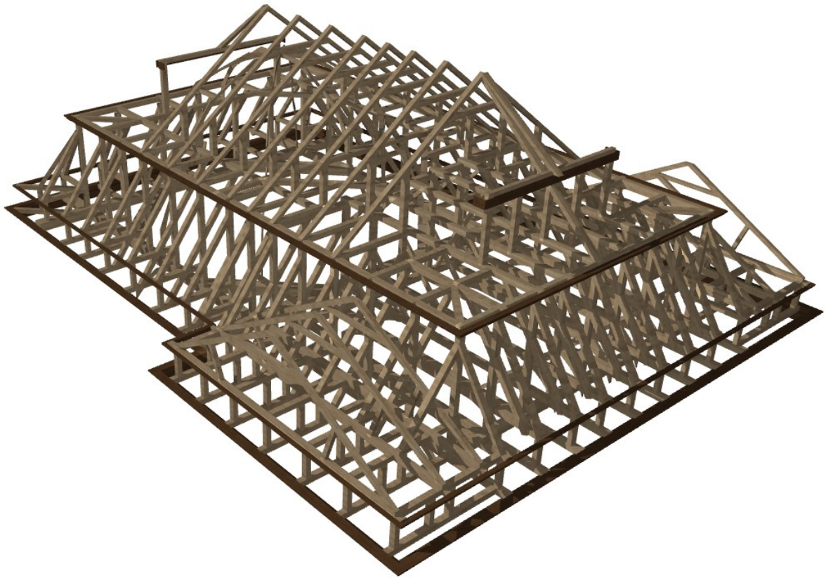
Fig. 146 Roof truss
