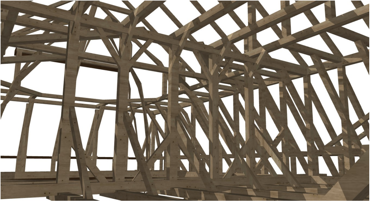
Fig. 148 Roof truss
