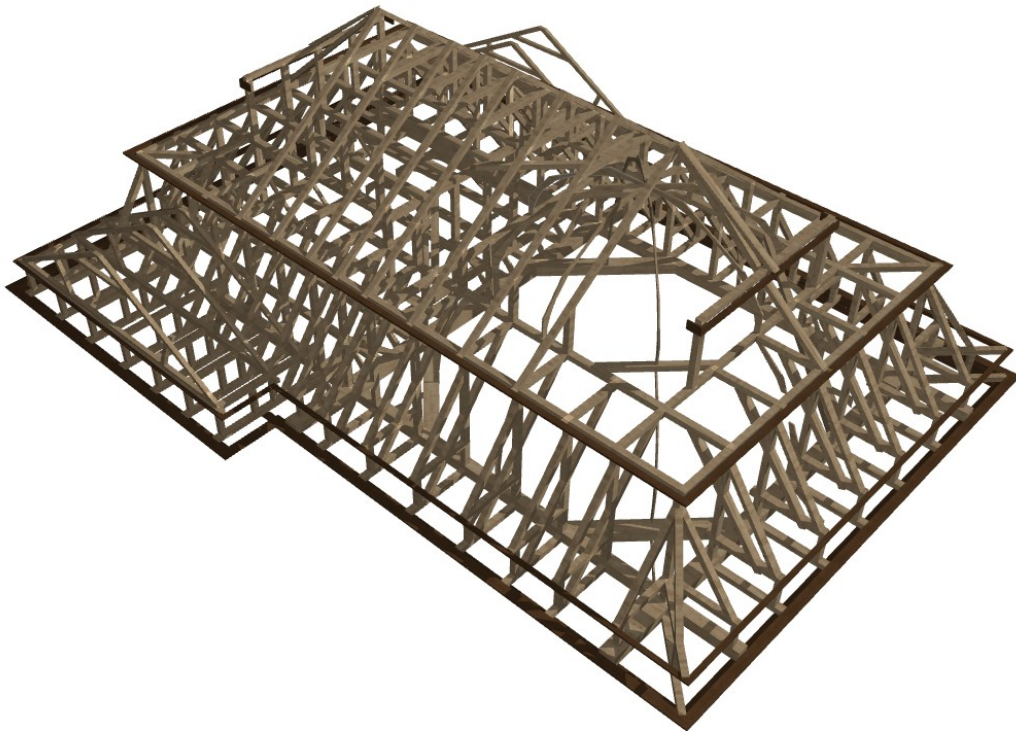
Fig. 147 Roof truss
