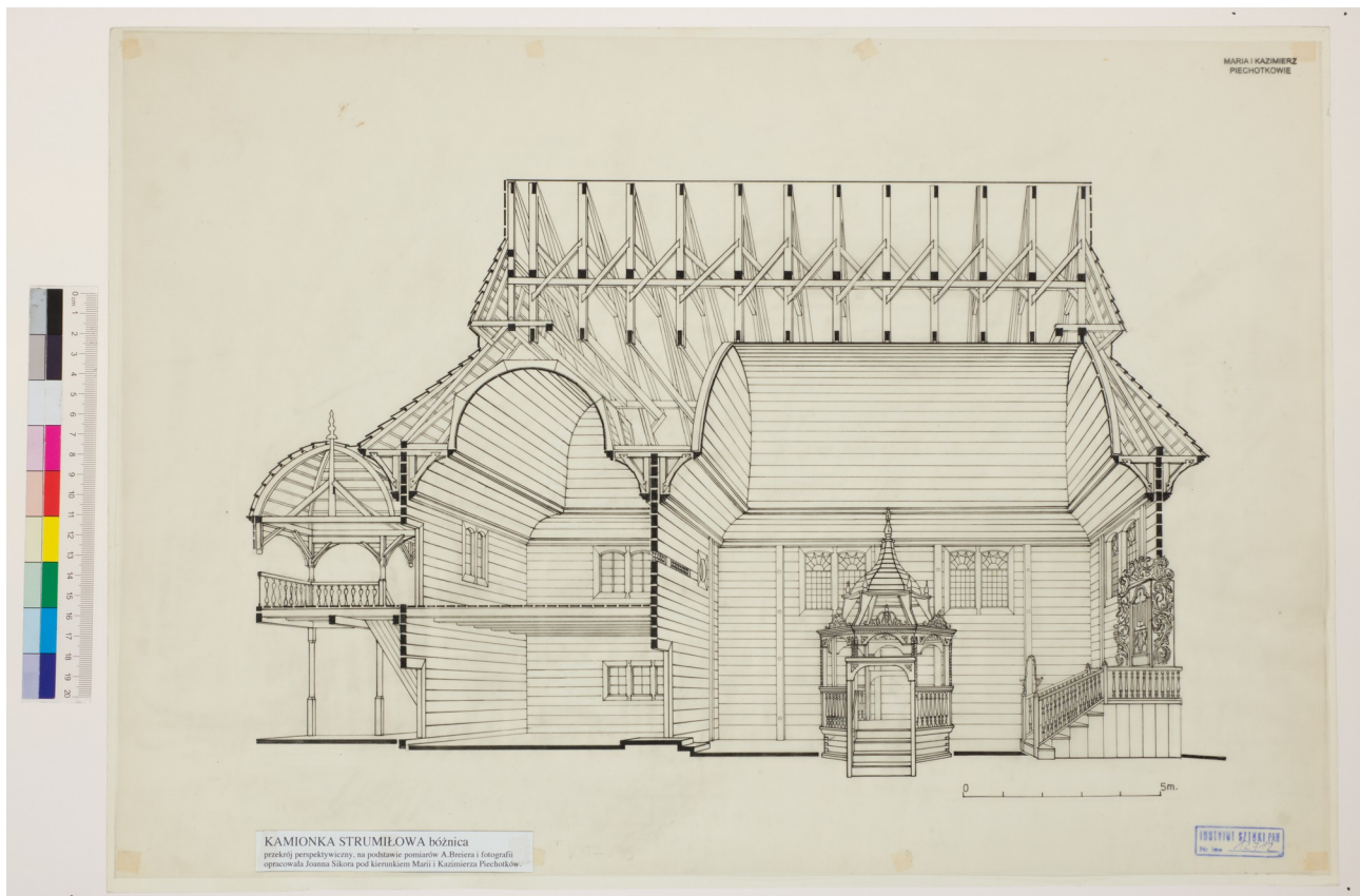
Fig. 1 Perspective Section
