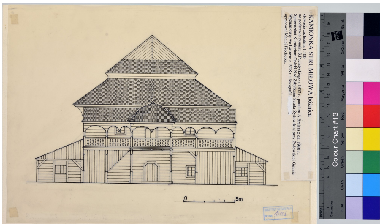
Fig. 5 Western Facade
